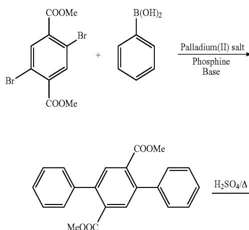
Synthesis scheme 1: Precursors of indenofluorene derivatives
