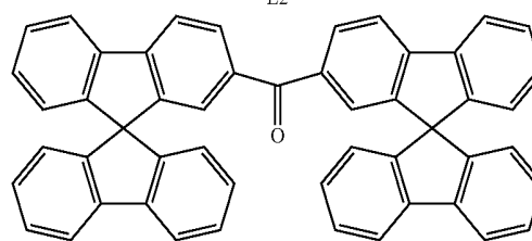
Bis(9,9'-spirobifluoren-2-yl) ketone (comparative material ketone 1)
